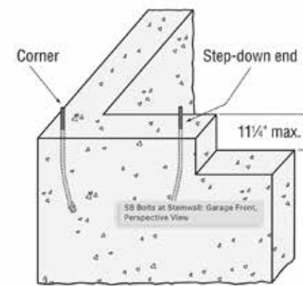
SB Bolts at Stemwall: Garage Front, Perspective View
